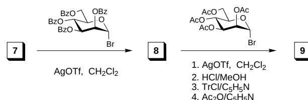
Scheme 4. Synthesis of the trityl ethers 8 and 9 .
