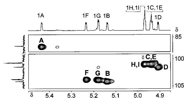
Figure 2. The anomeric region of the 2D-transformed data matrix from an HMQC experiment conducted on the nonasaccharide 29 (100 MHz, D 2 O, 25 °C). The assignment A/B/C/D/E/F/G/H/I of the D-mannopyranose residues is illustrated in Scheme 9.
