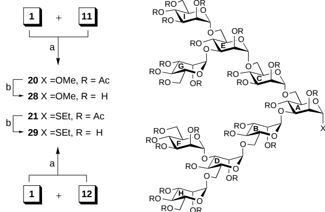
Scheme 9. Synthesis of the nonaosides 20 and 21 (and 28 and 29 ). Reagents and conditions: a) TrClO 4 (10 mol %), CH 2 Cl 2 , room temperature, 16 h, 50 % ( 20 ) and 54 % ( 21 ); b) NaOMe/MeOH/C 5 H 5 N.
