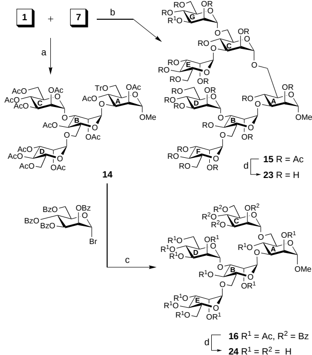
Scheme 6. Synthesis of the tetrasaccharide 14 , heptasaccharide 15 (and 23 ), and pentasaccharide 16 (and 24 ). Reagents and conditions: a) 1 (1 mol equiv), \text{TrClO}_4 (10 mol %), \text{CH}_2\text{Cl}_2 , room temperature, 16 h, 55%; b) 1 (2 mol equivalents), \text{TrClO}_4 (10 mol %), \text{CH}_2\text{Cl}_2 , room temperature, 16 h, 60%; c) 2,3,4,6-tetra- O -benzoyl- \alpha -D-mannopyranosyl bromide (4 equiv), \text{AgOTf/2,4,6-collidine} , \text{CH}_2\text{Cl}_2 , room temperature, 10 min (47%); d) \text{NaOMe/MeOH/C}_5\text{H}_5\text{N} .
