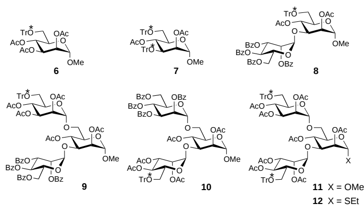
Scheme 3. Building blocks containing trityl ethers that can serve as glycosyl acceptors in reactions with the trisaccharide donor 1 . The potential sites of glycosylation are marked with asterisks.
