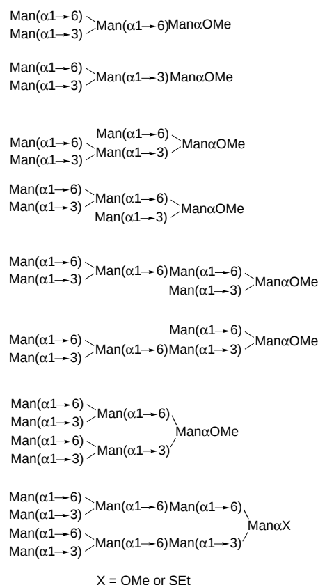
Scheme 1. Target branched-chain oligomannosides.
