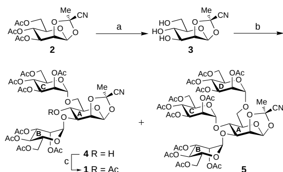
Scheme 2. Synthesis of the trisaccharide glycosyl donor 1 . Reagents and conditions: a) NaOMe/MeOH/C 5 H 5 N, room temperature, 5 min; b) 2,3,4,6-tetra- O -acetyl- \alpha -D-mannopyranosyl bromide, Hg(CN) 2 , HgBr 2 , MeCN, room temperature, 16 h (with 3.5 equiv of the glycosyl bromide the product is 4 , 62 %; with 4 equiv of the glycosyl bromide, the products after acetylation are 1 , 46 %, and 5 , 16 %); c) Ac 2 O/C 5 H 5 N, DMAP, 80 %.
