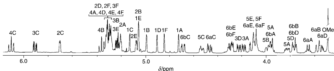
Figure 1. The “carbohydrate region” of the 1 H NMR spectrum (500 MHz, CDCl 3 , 20 °C) of the hexasaccharide derivative 19 showing the assignments of all the resonances. The designation of the monosaccharide residues ( A – F ) in 19 is shown in Scheme 8.
