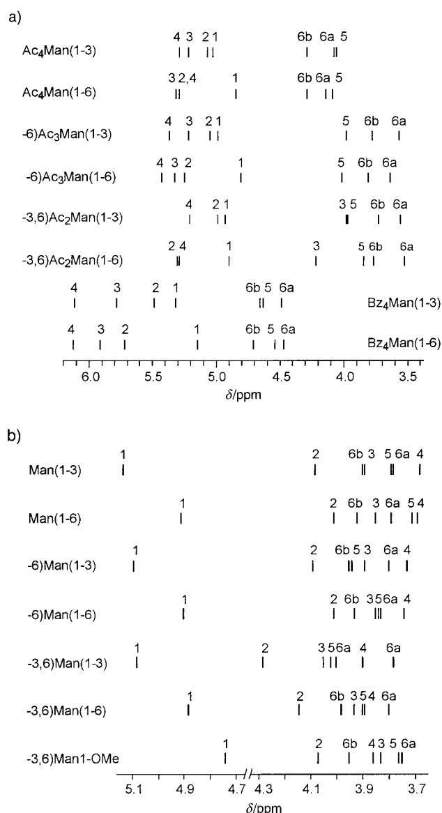
Figure 3. A schematic representation of 1 H NMR spectroscopic data for some typical \alpha -D-mannopyranose residues incorporated into a) protected and b) deprotected 3,6-branched mannooligosaccharides. Chemical shifts are depicted as vertical lines and their values are calculated as the means of \delta values for the analogous signals in similar residues selected from Tables 2 and 4.
