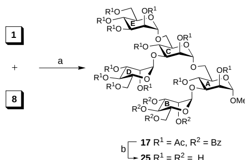
Scheme 7. Synthesis of the pentaoside 17 (and 25 ). Reagents and conditions: a) \text{TrClO}_4 (10 mol %), \text{CH}_2\text{Cl}_2 , room temperature, 16 h, 66%; b) \text{NaOMe/MeOH/C}_5\text{H}_5\text{N} .
