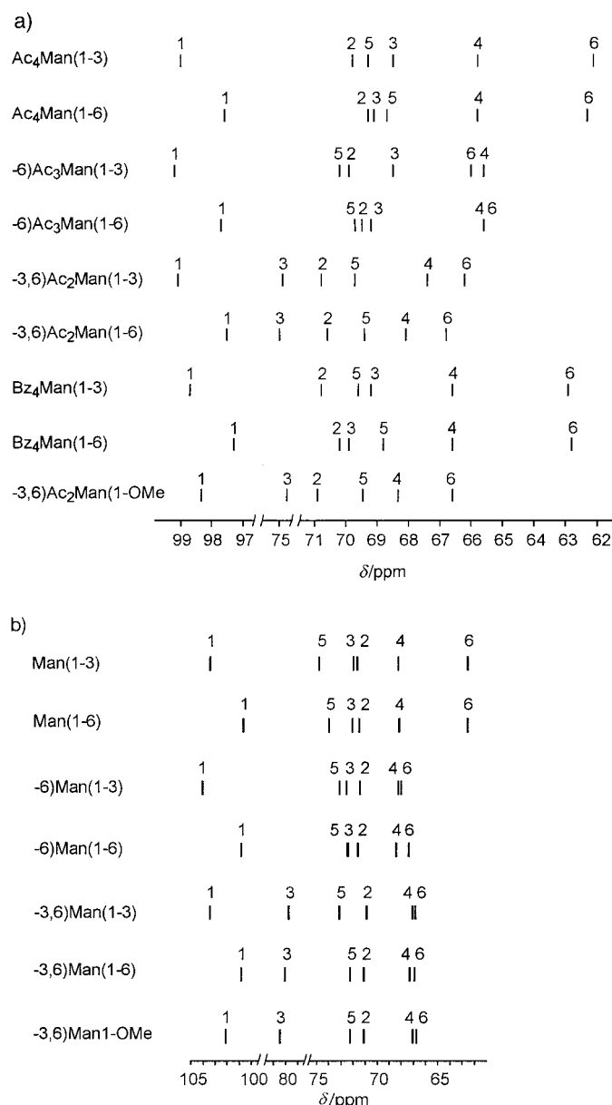
Figure 4. A schematic representation of ^{13}\text{C} NMR spectroscopic data for some typical \alpha -D-mannopyranose residues incorporated into a) protected and b) deprotected 3,6-branched mannoooligosaccharides. Chemical shifts are depicted as vertical lines and their values are calculated as the means of \delta values for the analogous signals in similar residues selected from Tables 3 and 5.
