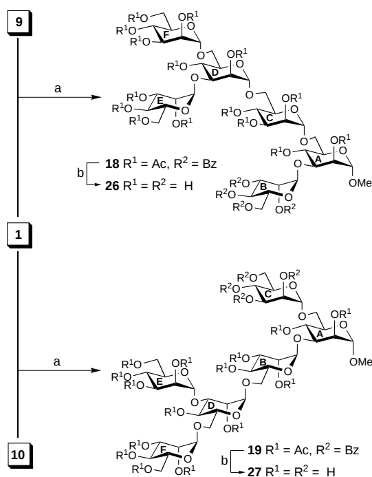
Scheme 8. Synthesis of the isomeric hexaosides 18 and 19 (and 26 and 27 ). Reagents and conditions: a) TrClO 4 (10 mol %), CH 2 Cl 2 , room temperature, 16 h, 58 % ( 18 ) and 60 % ( 19 ); b) NaOMe/MeOH.
